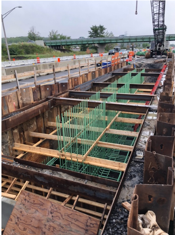
Median pier footing rebar
