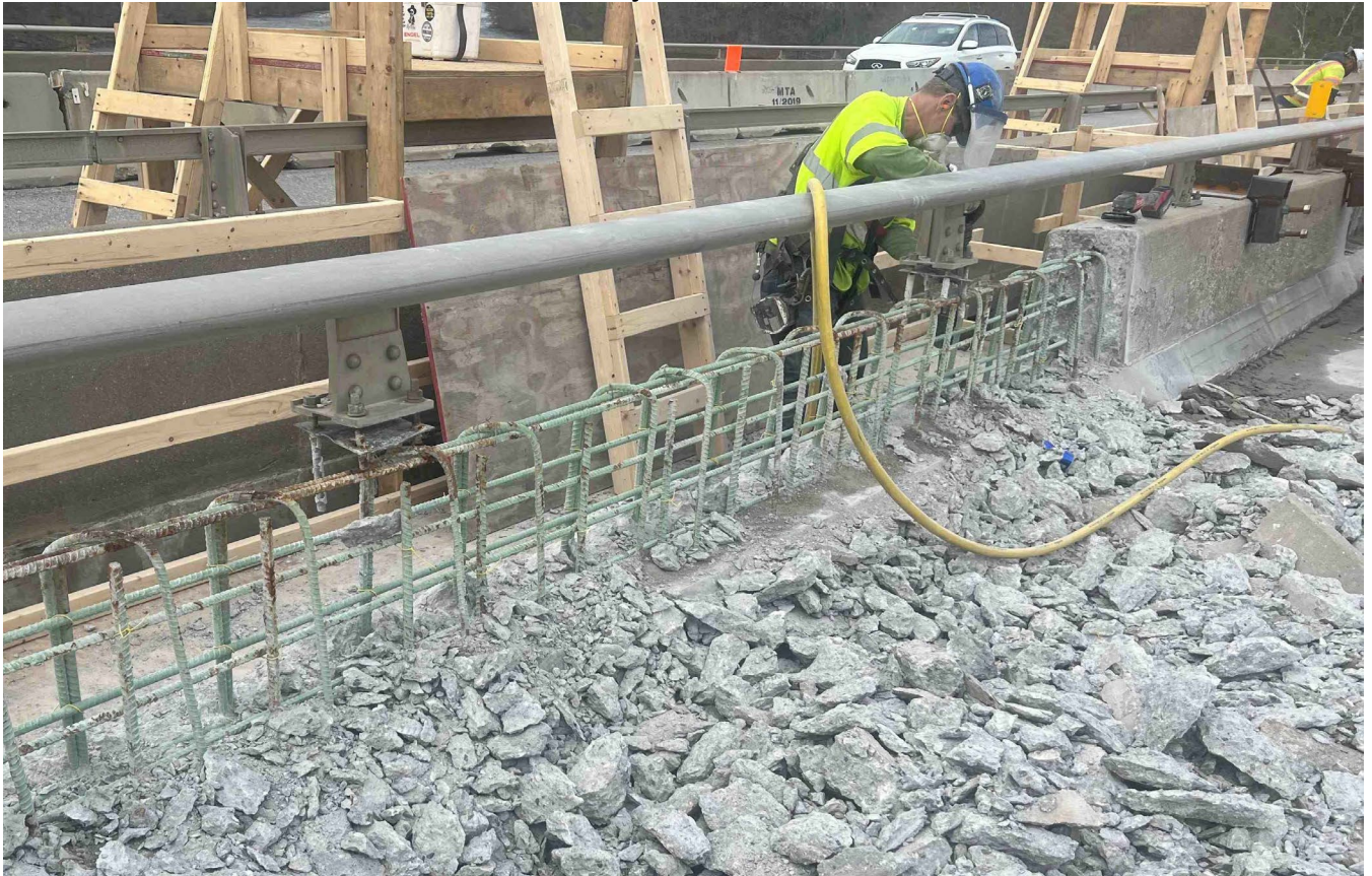
Crews work diligently to remove failing concrete in the northbound parapet
